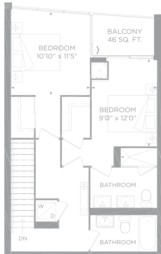
UPPER LEVEL
