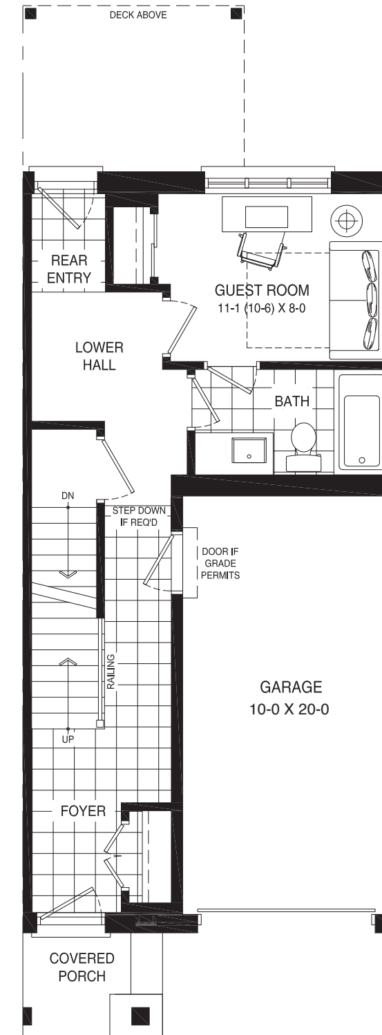
OPT. GROUND FLOOR
